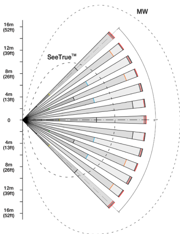
TOP VIEW (Forward Detector)
